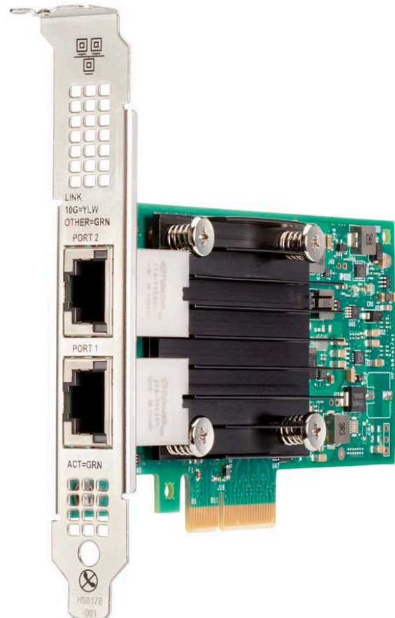
HPE Ethernet 10Gb 2-port 562T Adapter
