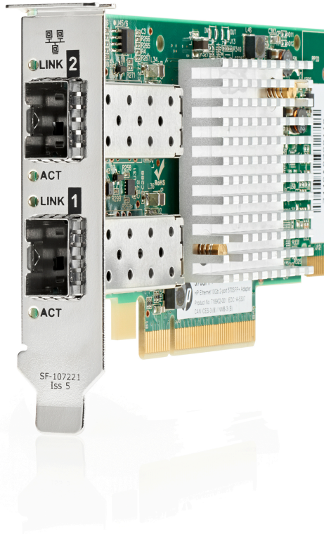
HPE Ethernet 10Gb 2-port 571SFP+ Adapter with the low profile bracket
